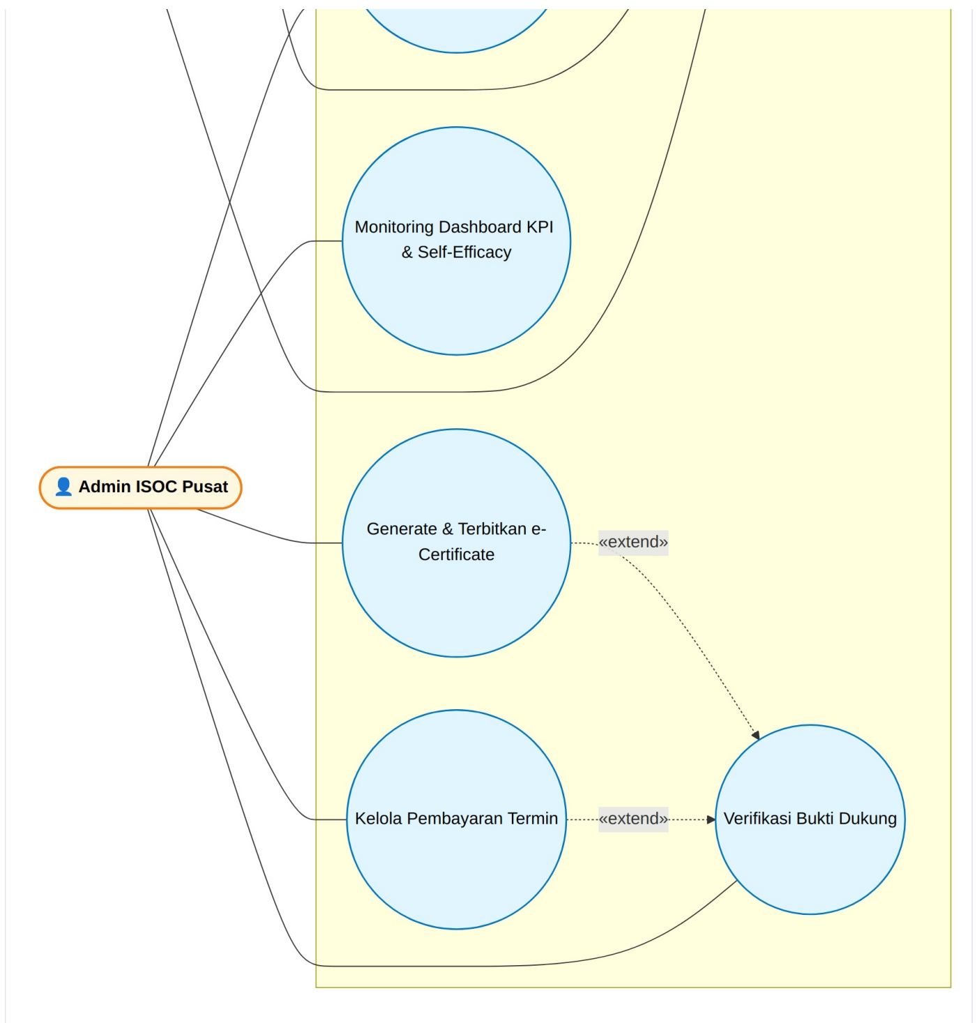
Use Case Diagram SI-DSC
